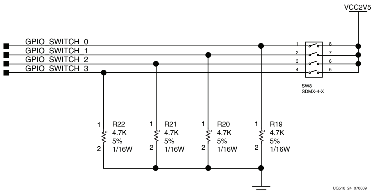
Figure 1-12: User DIP Switch
