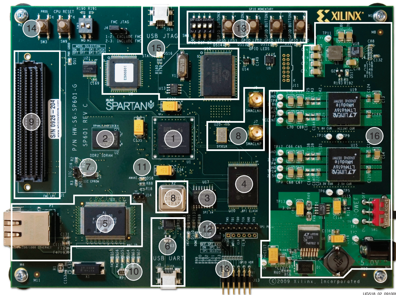
Figure 1-2: SP601 Board Photo
