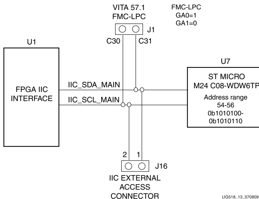
Figure 1-6: IIC Bus Topology
