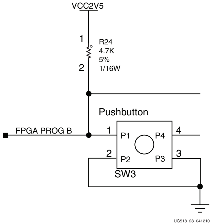
Figure 1-15: FPGA_PROG_B Pushbutton Switch Topology
