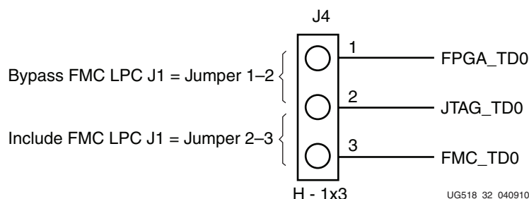
Figure 1-17: VITA 57.1 FMC JTAG Bypass Jumper
