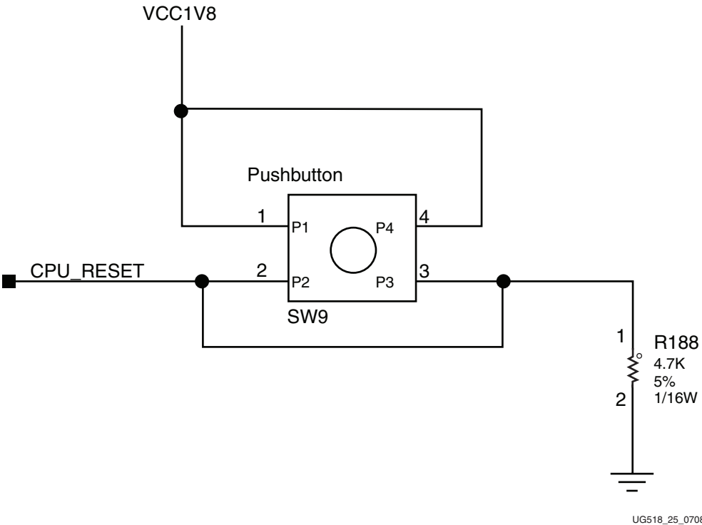
Figure 1-13: User Pushbutton Switch (Typical)
