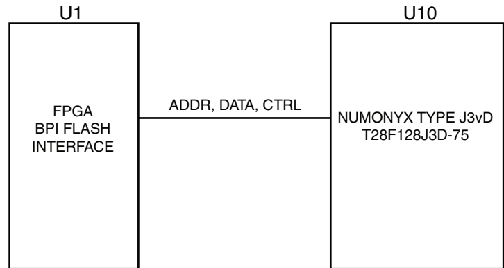
Figure 1-5: Linear Flash BPI Interface
