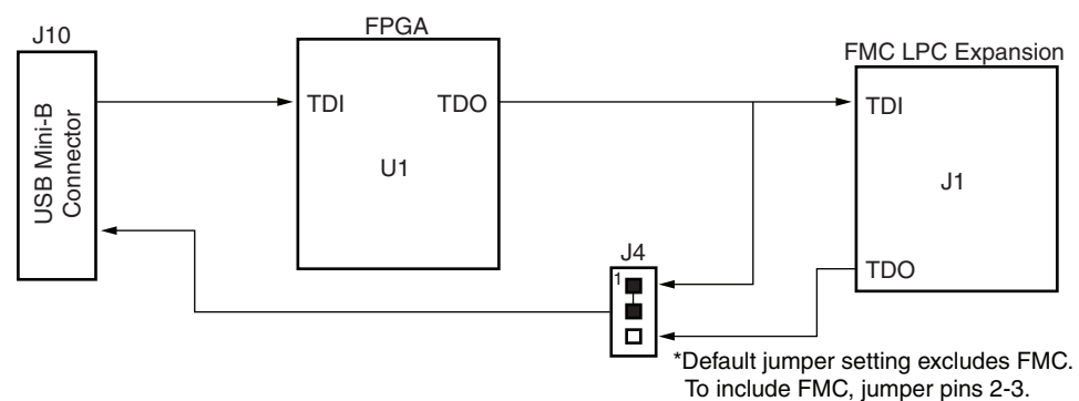
Figure 1-16: JTAG Chain
