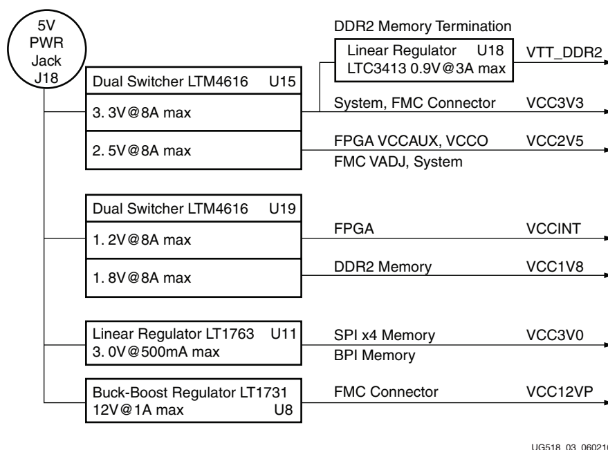
Figure 1-18: Power Supply
