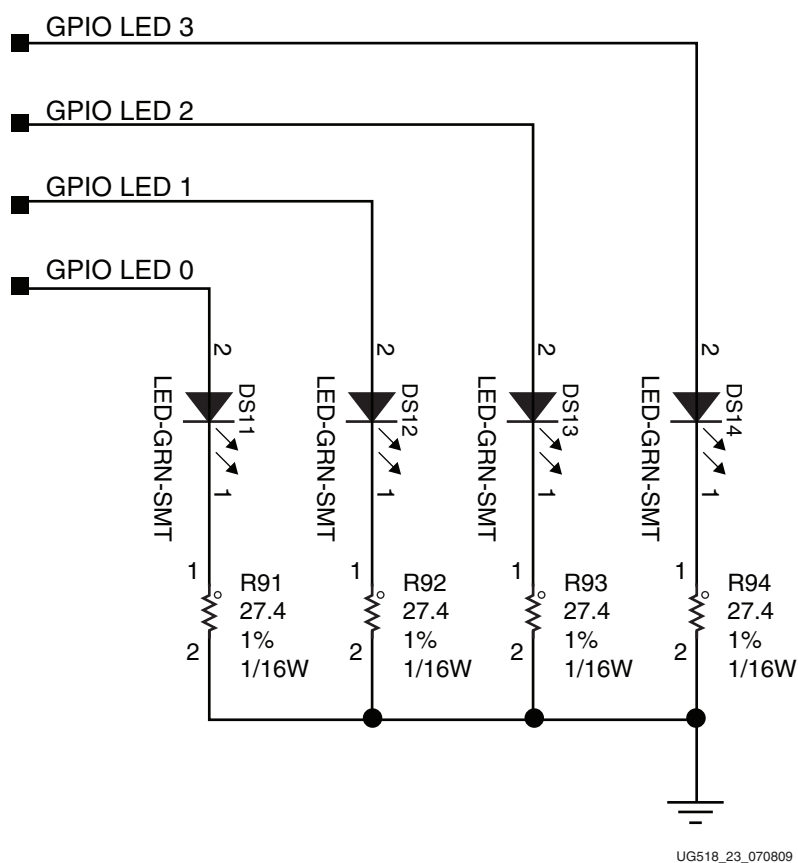
Figure 1-11: User LEDs
