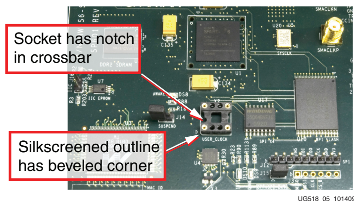
Figure 1-7: SP601 Oscillator Socket Pin 1 Location Identifiers
